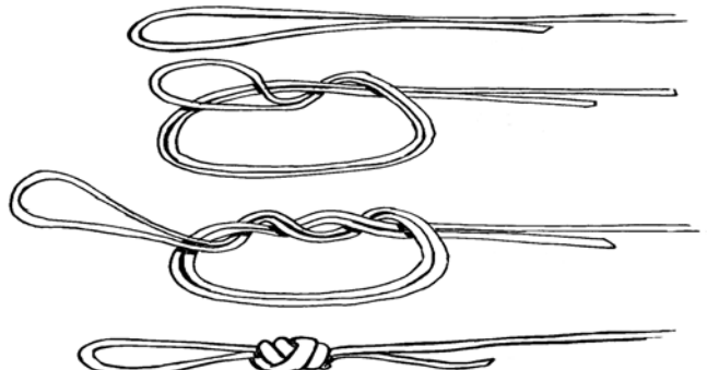
Surgeon's/Double-Overhand (Loop to Loop Connections)
