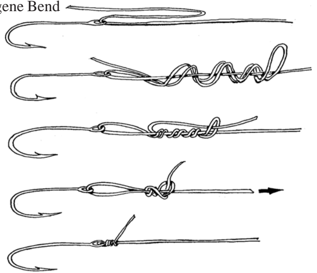
Fly To Leader/Tippet
