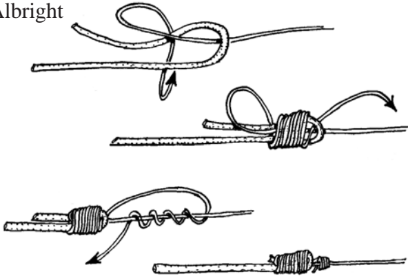
Backing To Flyline
